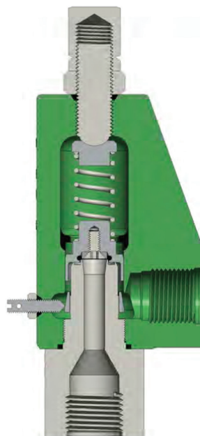
F85M 'M' (Micro) Body - HP Block F85M-4 w/ SAE AS5202 connections shown
