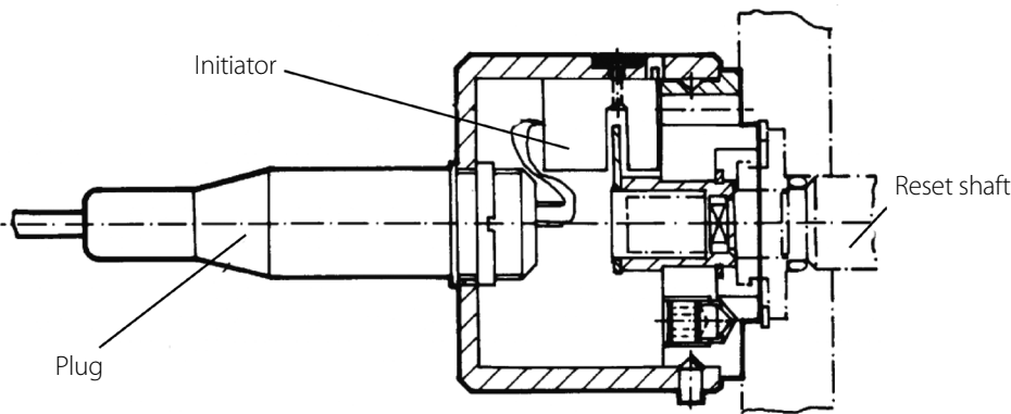
SSV position indicator for assembly* at the reset shaft, *order technical information No. 142-099-6001
